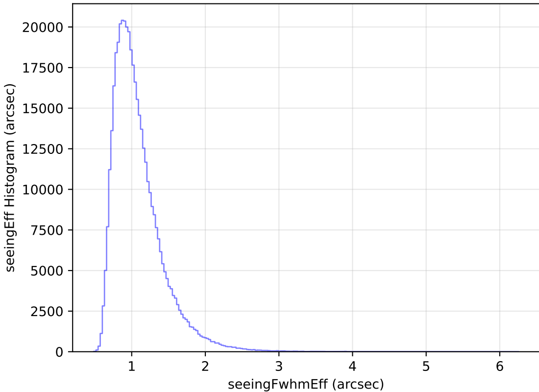
too_elab_r32_d2_griz_v3.4_10yrs WFD z band: seeingEff Histogram
