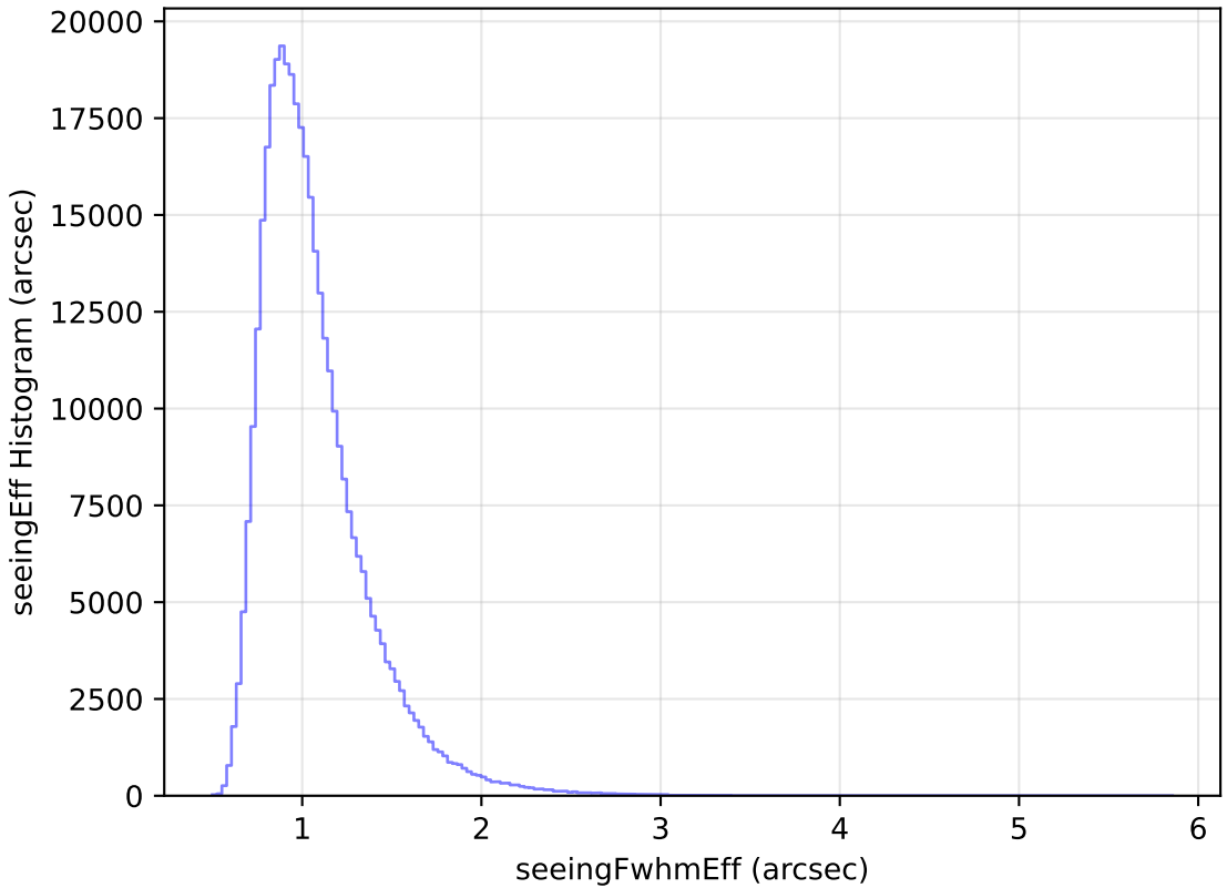
too_elab_r32_d2_griz_v3.4_10yrs WFD y band: seeingEff Histogram
