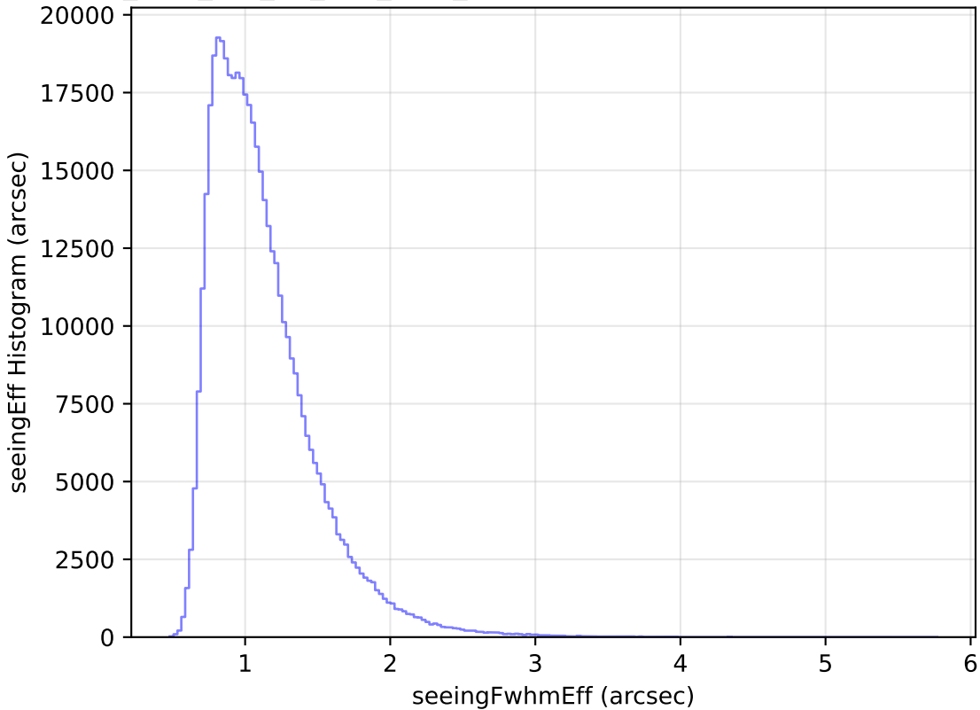
too_elab_r32_d2_griz_v3.4_10yrs WFD r band: seeingEff Histogram
