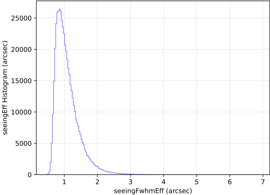
too_elab_r32_d2_griz_v3.4_10yrs WFD i band: seeingEff Histogram
