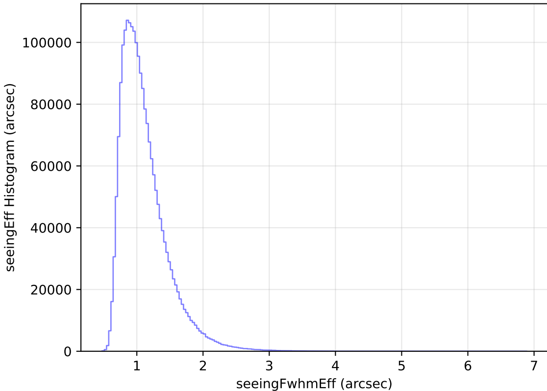
too_elab_r32_d2_griz_v3.4_10yrs WFD all bands: seeingEff Histogram
