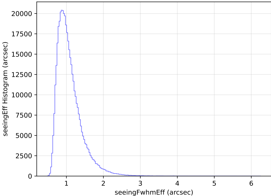
too_elab_r32_d2_griz_v3.4_10yrs All sky z band: seeingEff Histogram
