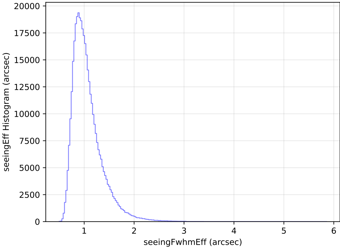
too_elab_r32_d2_griz_v3.4_10yrs All sky y band: seeingEff Histogram
