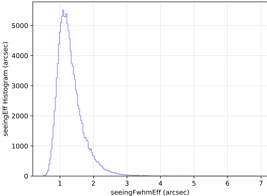
too_elab_r32_d2_griz_v3.4_10yrs All sky u band: seeingEff Histogram
