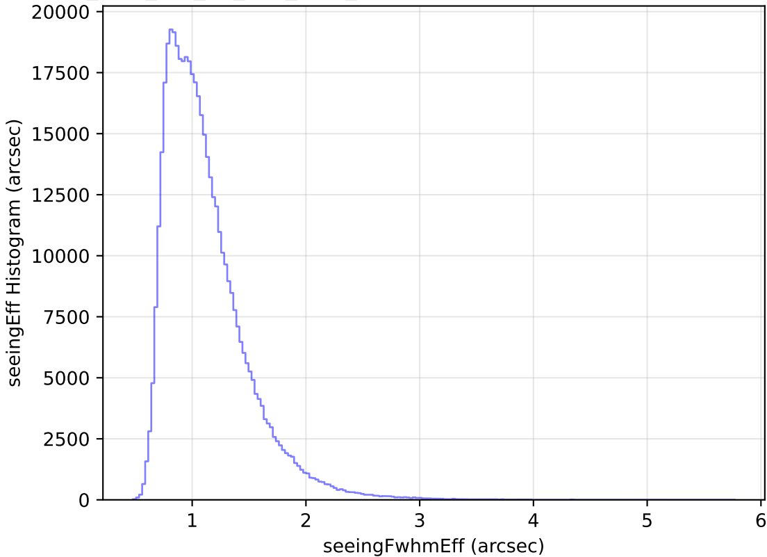
too_elab_r32_d2_griz_v3.4_10yrs All sky r band: seeingEff Histogram
