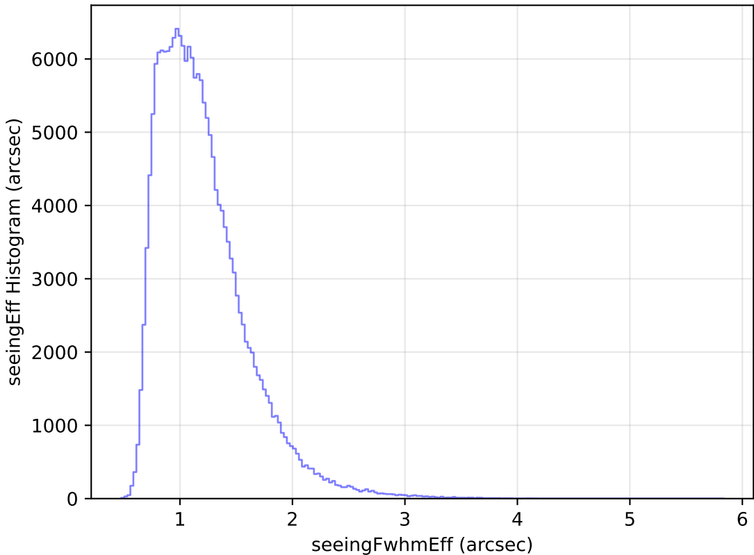
too_elab_r32_d2_griz_v3.4_10yrs All sky g band: seeingEff Histogram
