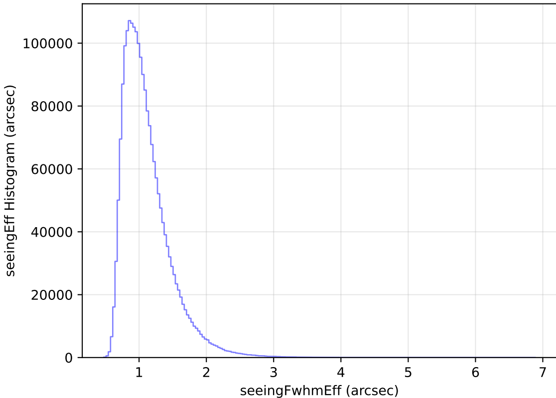
too_elab_r32_d2_griz_v3.4_10yrs All sky all bands: seeingEff Histogram
