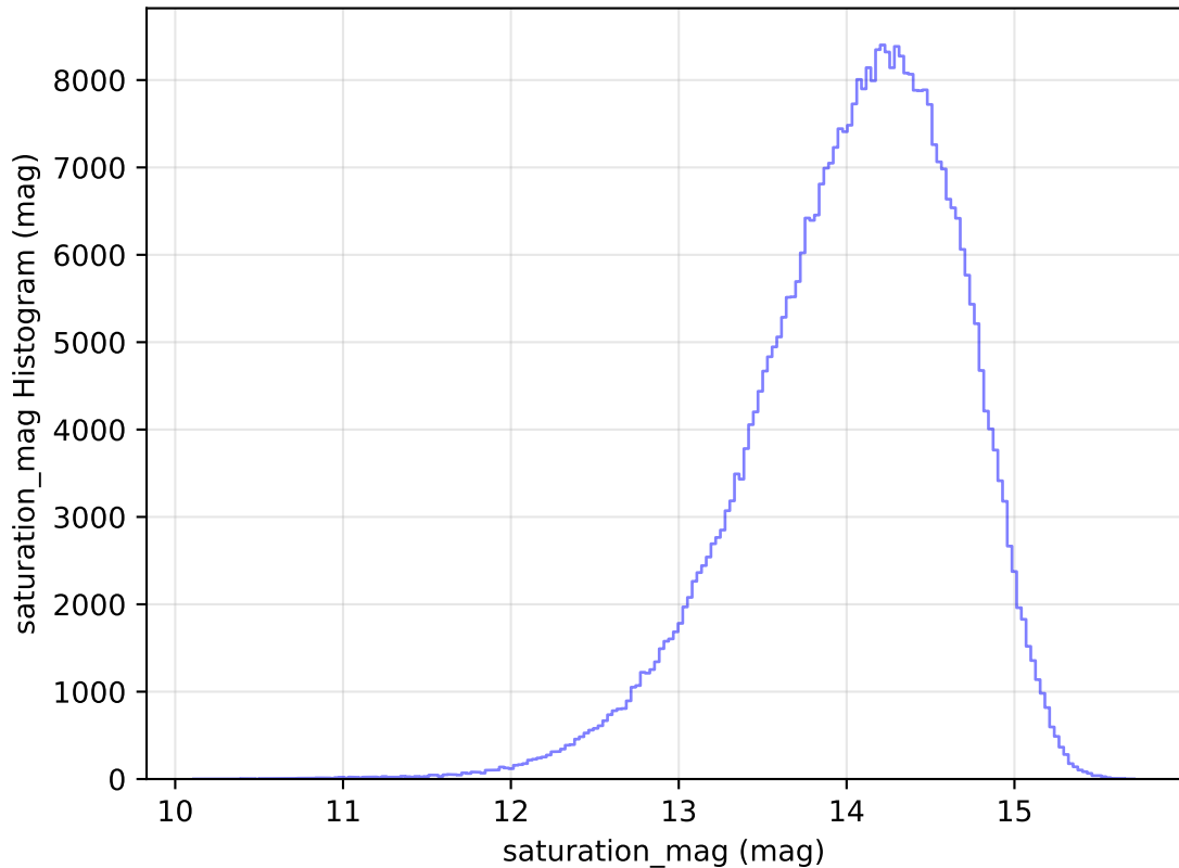
too_elab_r32_d2_griz_v3.4_10yrs WFD z band: saturation_mag Histogram
