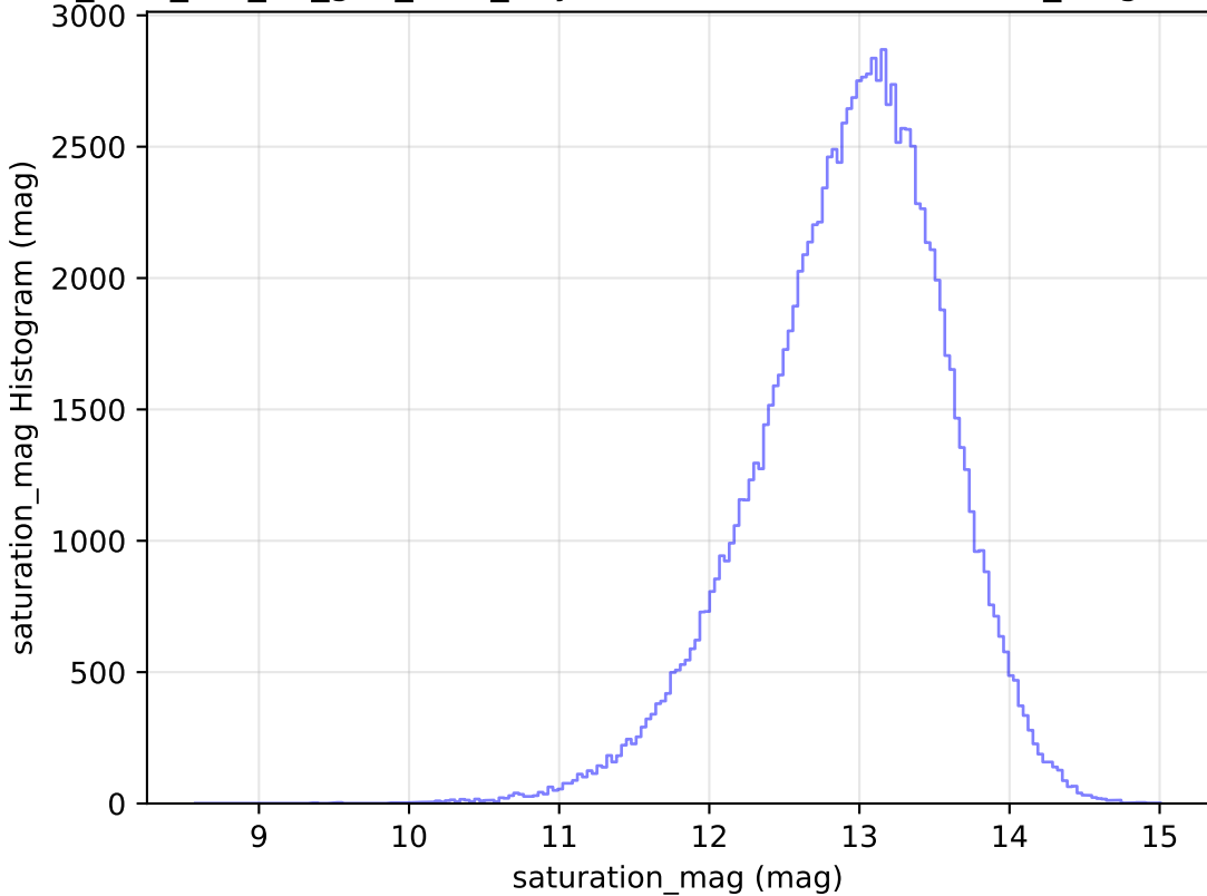
too_elab_r32_d2_griz_v3.4_10yrs WFD u band: saturation_mag Histogram
