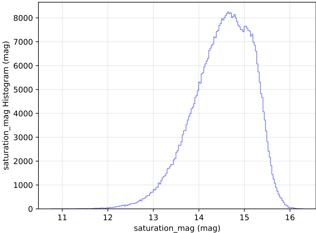
too_elab_r32_d2_griz_v3.4_10yrs WFD r band: saturation_mag Histogram
