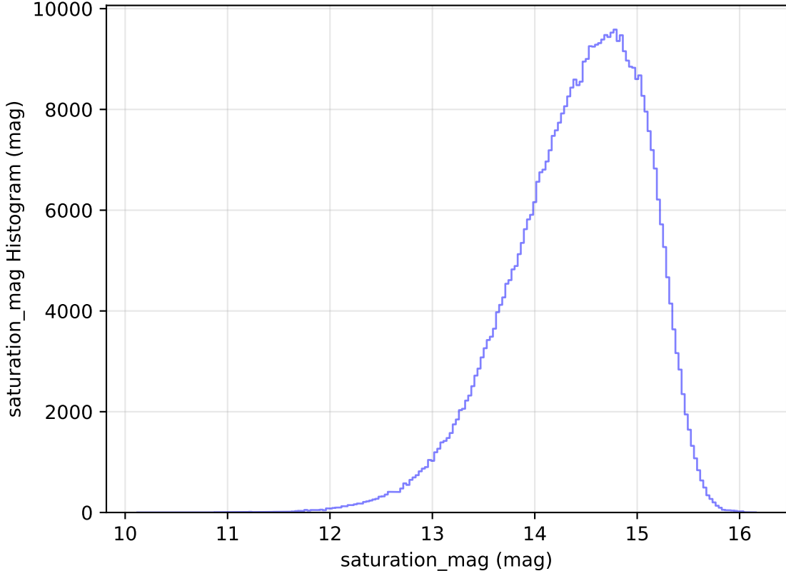
too_elab_r32_d2_griz_v3.4_10yrs WFD i band: saturation_mag Histogram
