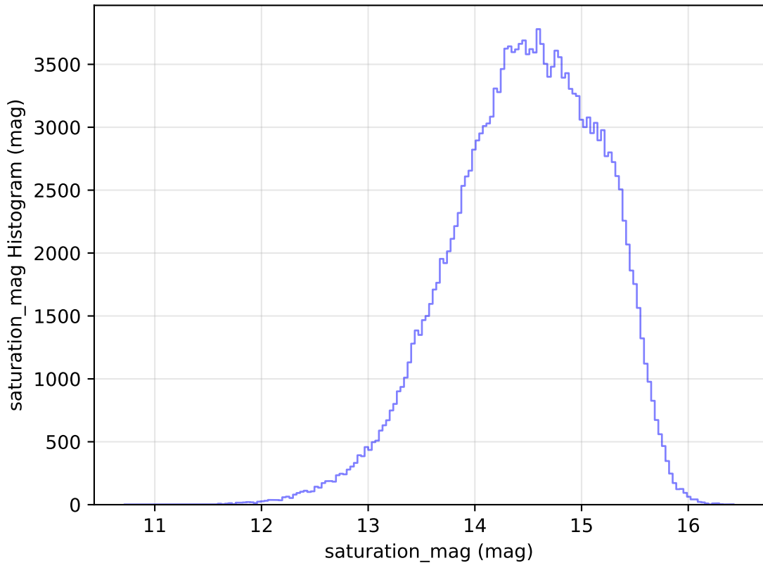
too_elab_r32_d2_griz_v3.4_10yrs WFD g band: saturation_mag Histogram
