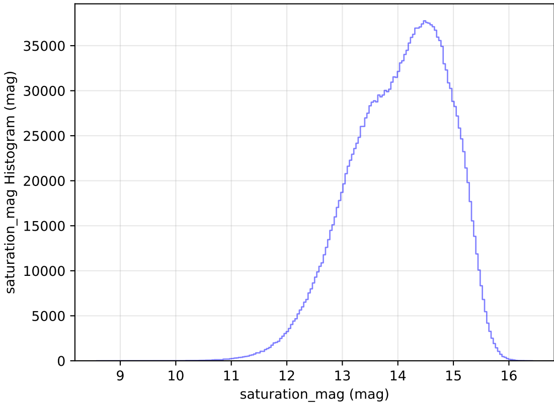
too_elab_r32_d2_griz_v3.4_10yrs WFD all bands: saturation_mag Histogram
