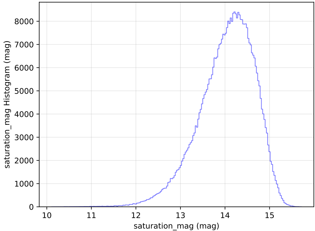
too_elab_r32_d2_griz_v3.4_10yrs All sky z band: saturation_mag Histogram
