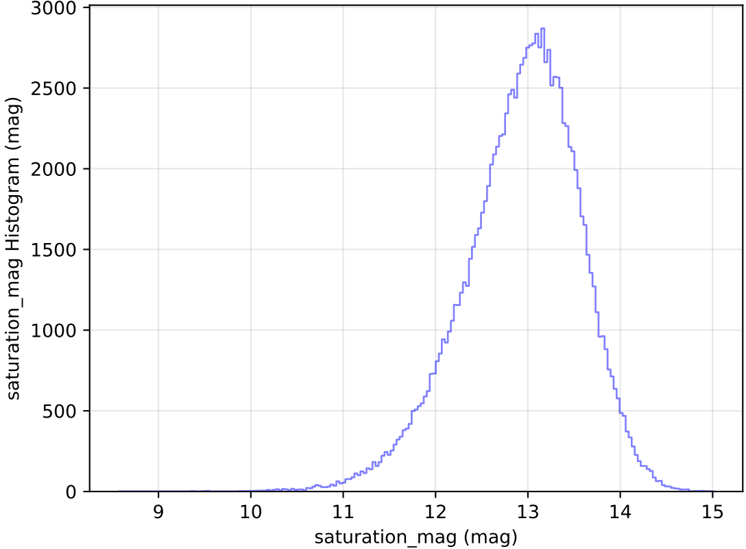
too_elab_r32_d2_griz_v3.4_10yrs All sky u band: saturation_mag Histogram
