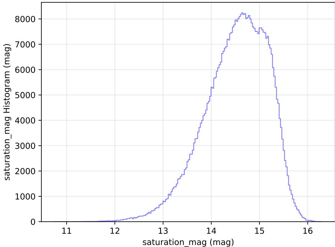
too_elab_r32_d2_griz_v3.4_10yrs All sky r band: saturation_mag Histogram
