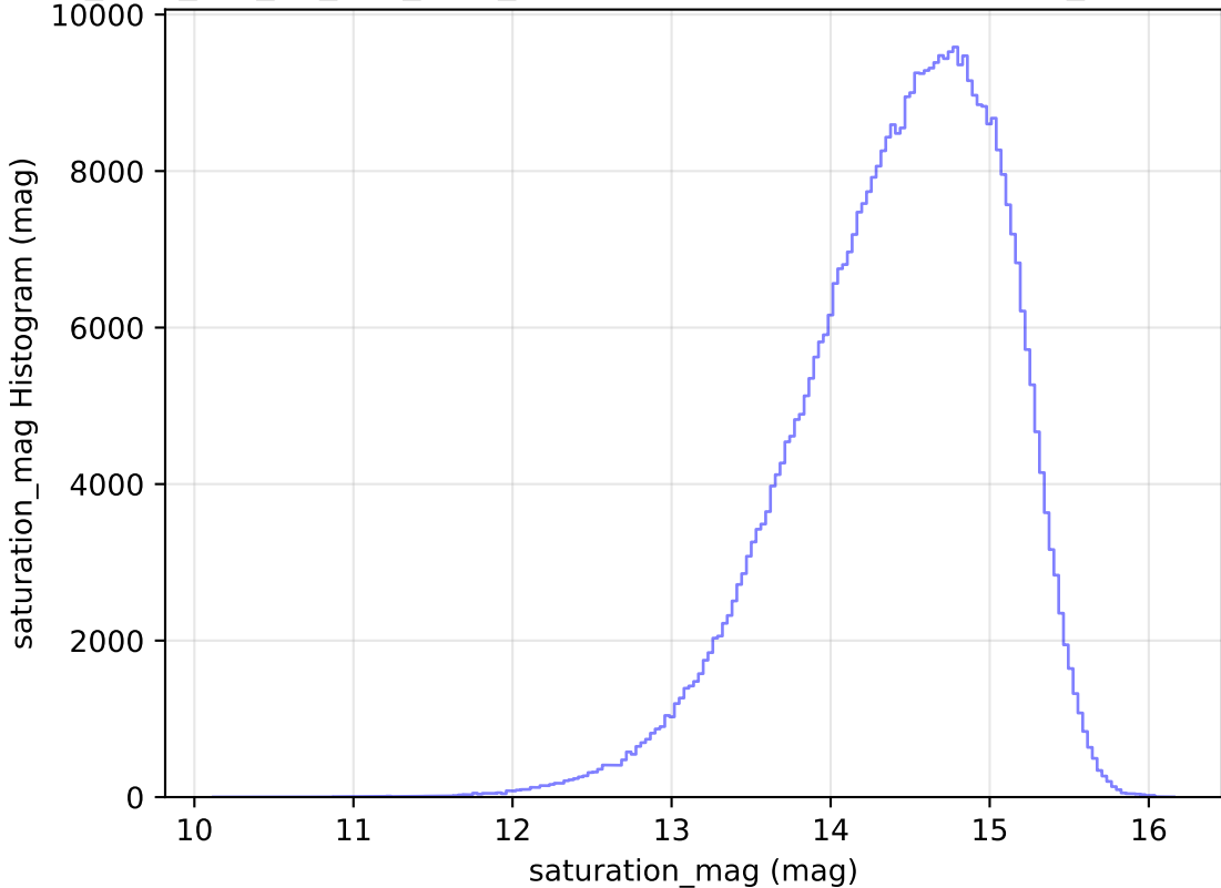
too_elab_r32_d2_griz_v3.4_10yrs All sky i band: saturation_mag Histogram
