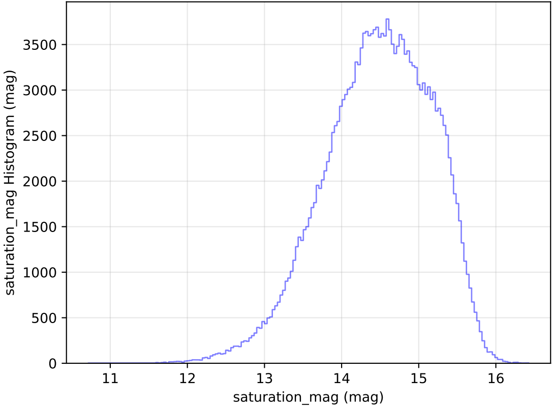
too_elab_r32_d2_griz_v3.4_10yrs All sky g band: saturation_mag Histogram
