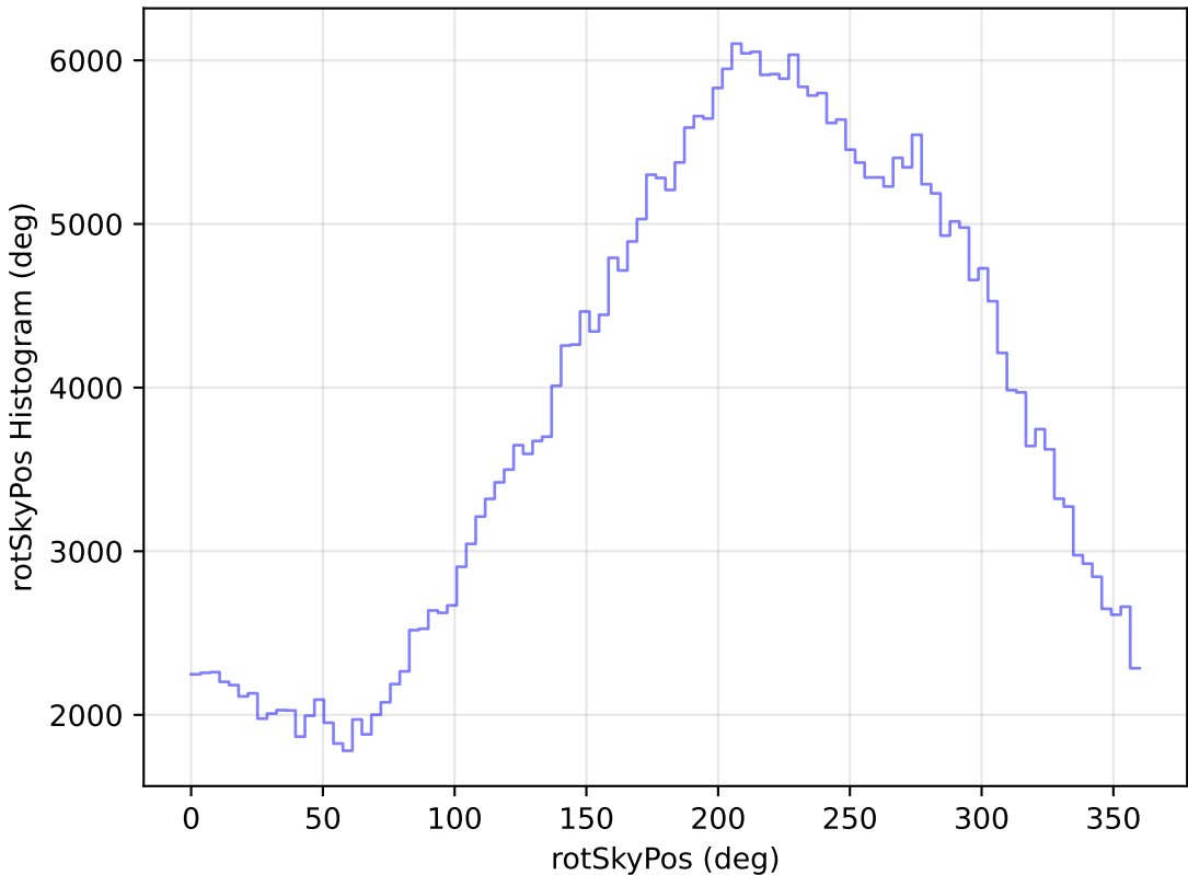
too_elab_r32_d2_griz_v3.4_10yrs WFD y band: rotSkyPos Histogram
