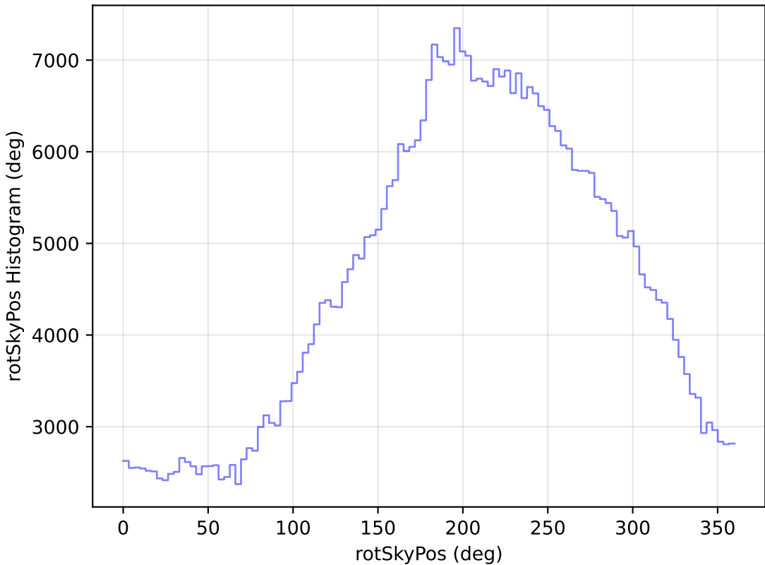
too_elab_r32_d2_griz_v3.4_10yrs WFD i band: rotSkyPos Histogram
