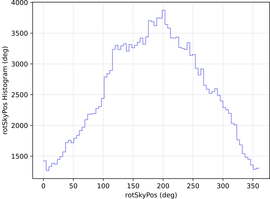
too_elab_r32_d2_griz_v3.4_10yrs WFD g band: rotSkyPos Histogram
