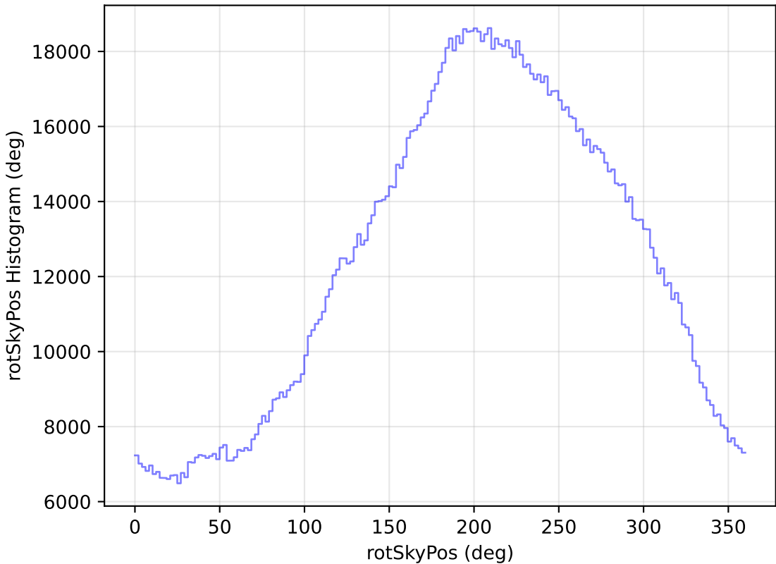
too_elab_r32_d2_griz_v3.4_10yrs WFD all bands: rotSkyPos Histogram
