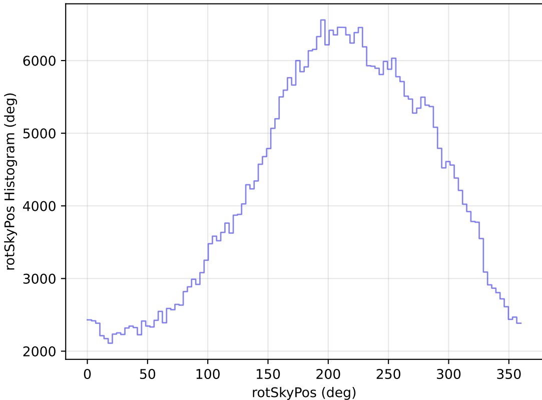
too_elab_r32_d2_griz_v3.4_10yrs All sky z band: rotSkyPos Histogram
