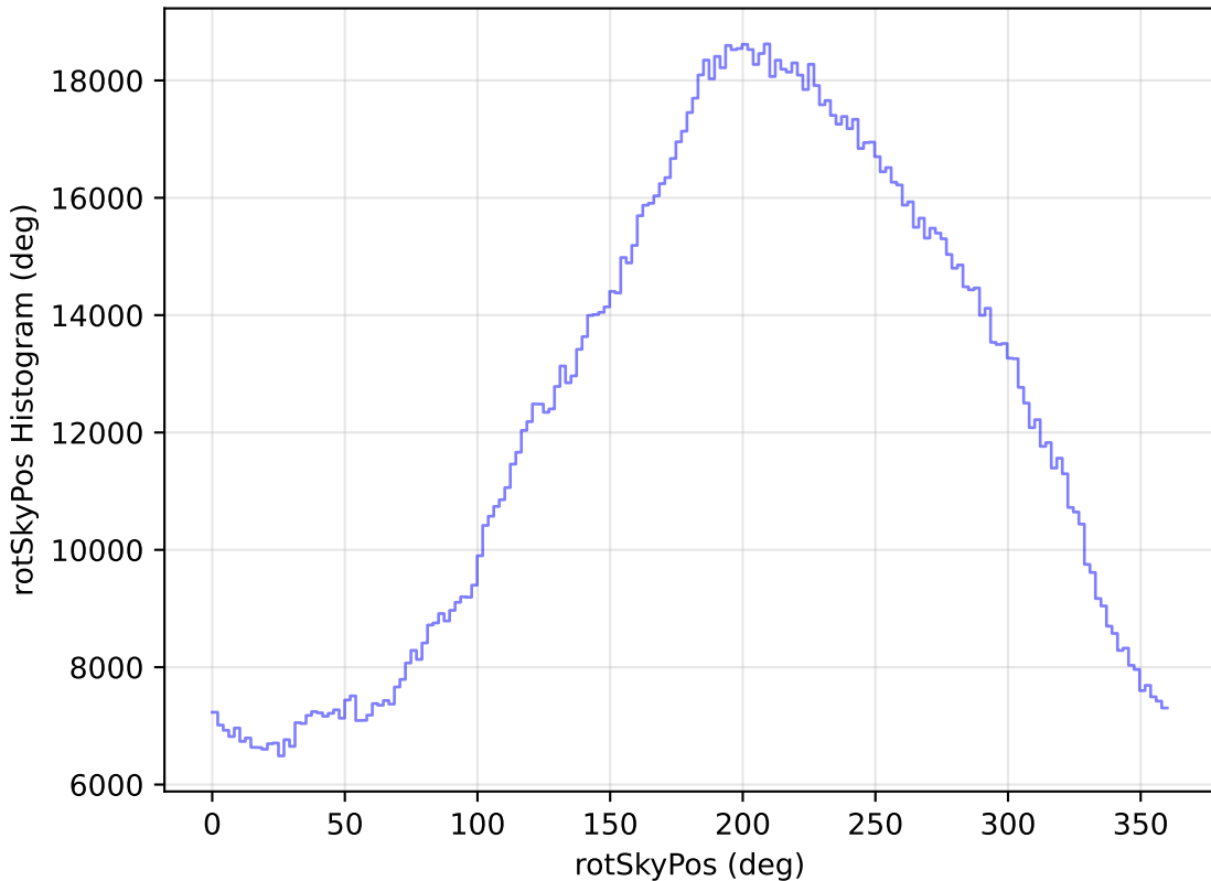
too_elab_r32_d2_griz_v3.4_10yrs All sky all bands: rotSkyPos Histogram
