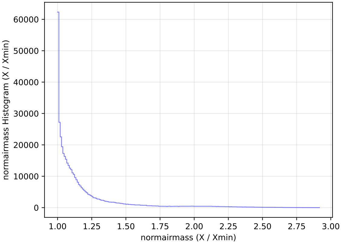
too_elab_r32_d2_griz_v3.4_10yrs WFD z band: normairmass Histogram
