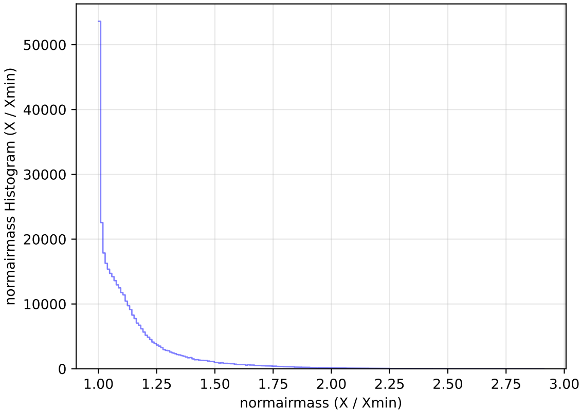
too_elab_r32_d2_griz_v3.4_10yrs WFD y band: normairmass Histogram
