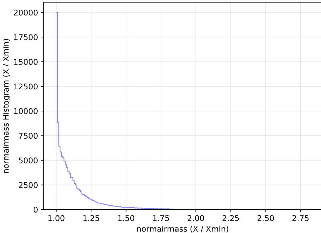
too_elab_r32_d2_griz_v3.4_10yrs WFD u band: normairmass Histogram
