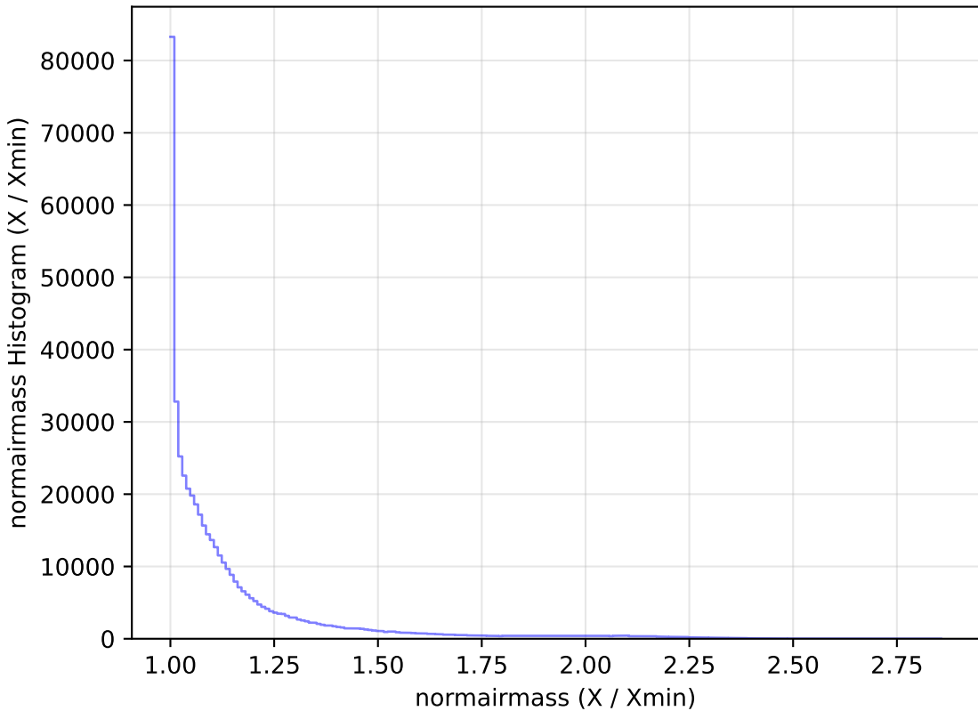
too_elab_r32_d2_griz_v3.4_10yrs WFD r band: normairmass Histogram
