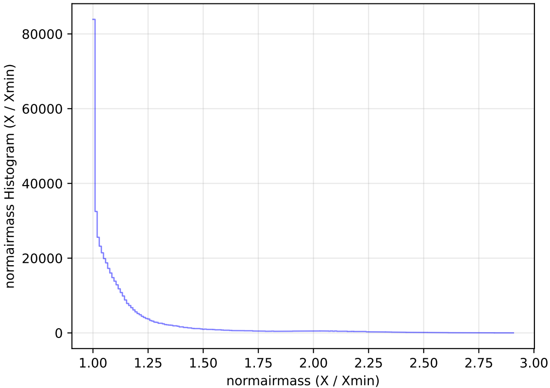
too_elab_r32_d2_griz_v3.4_10yrs WFD i band: normairmass Histogram
