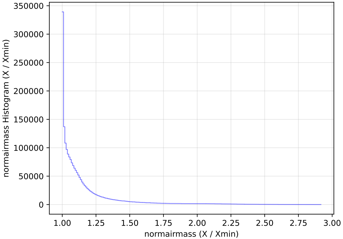
too_elab_r32_d2_griz_v3.4_10yrs WFD all bands: normairmass Histogram
