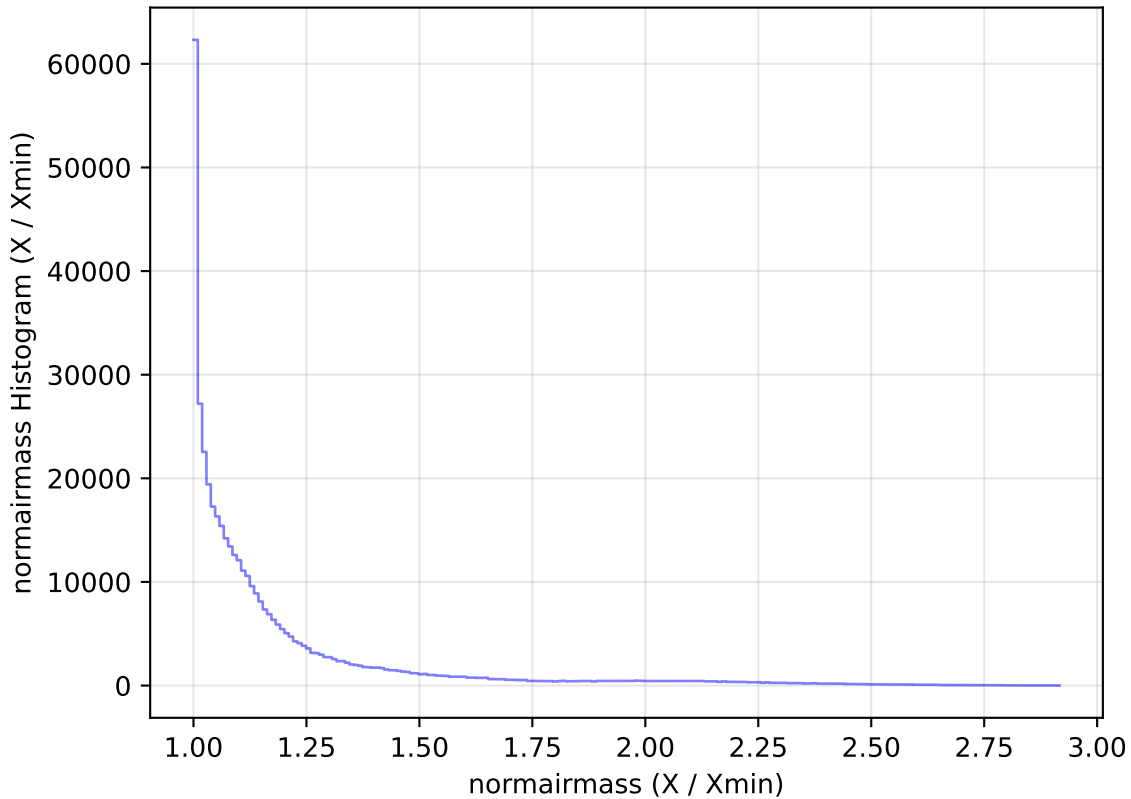
too_elab_r32_d2_griz_v3.4_10yrs All sky z band: normairmass Histogram
