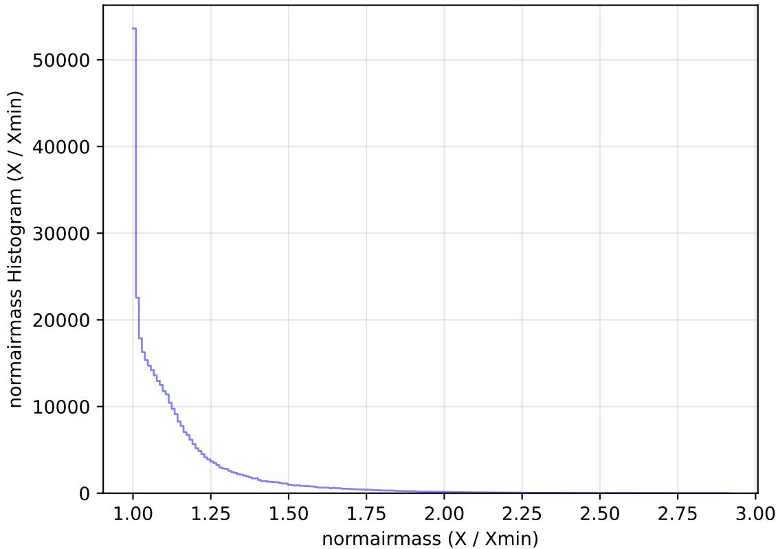
too_elab_r32_d2_griz_v3.4_10yrs All sky y band: normairmass Histogram
