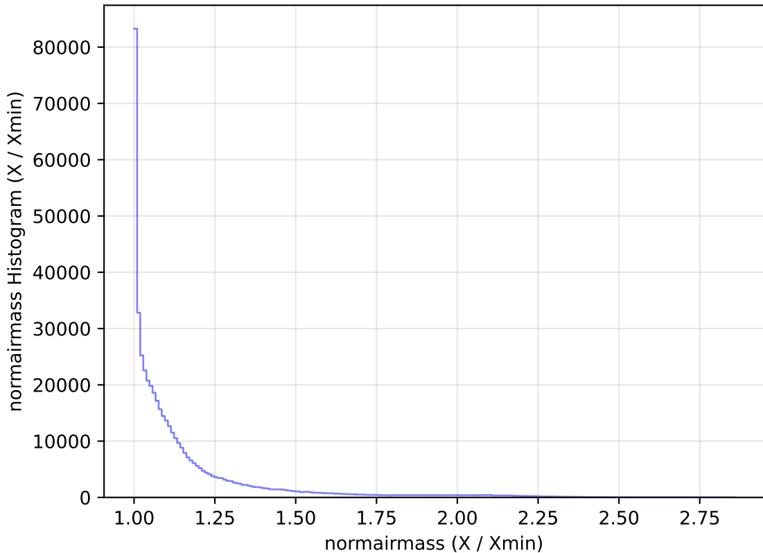
too_elab_r32_d2_griz_v3.4_10yrs All sky r band: normairmass Histogram
