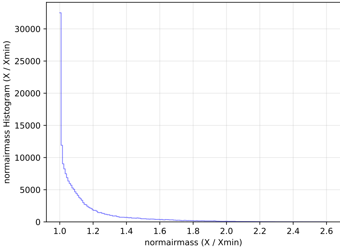
too_elab_r32_d2_griz_v3.4_10yrs All sky g band: normairmass Histogram
