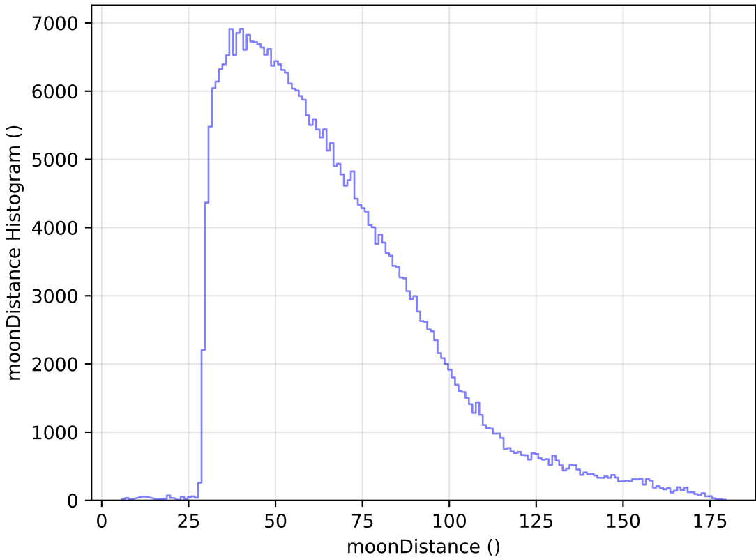
too_elab_r32_d2_griz_v3.4_10yrs WFD y band: moonDistance Histogram
