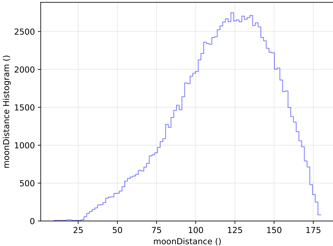
too_elab_r32_d2_griz_v3.4_10yrs WFD u band: moonDistance Histogram
