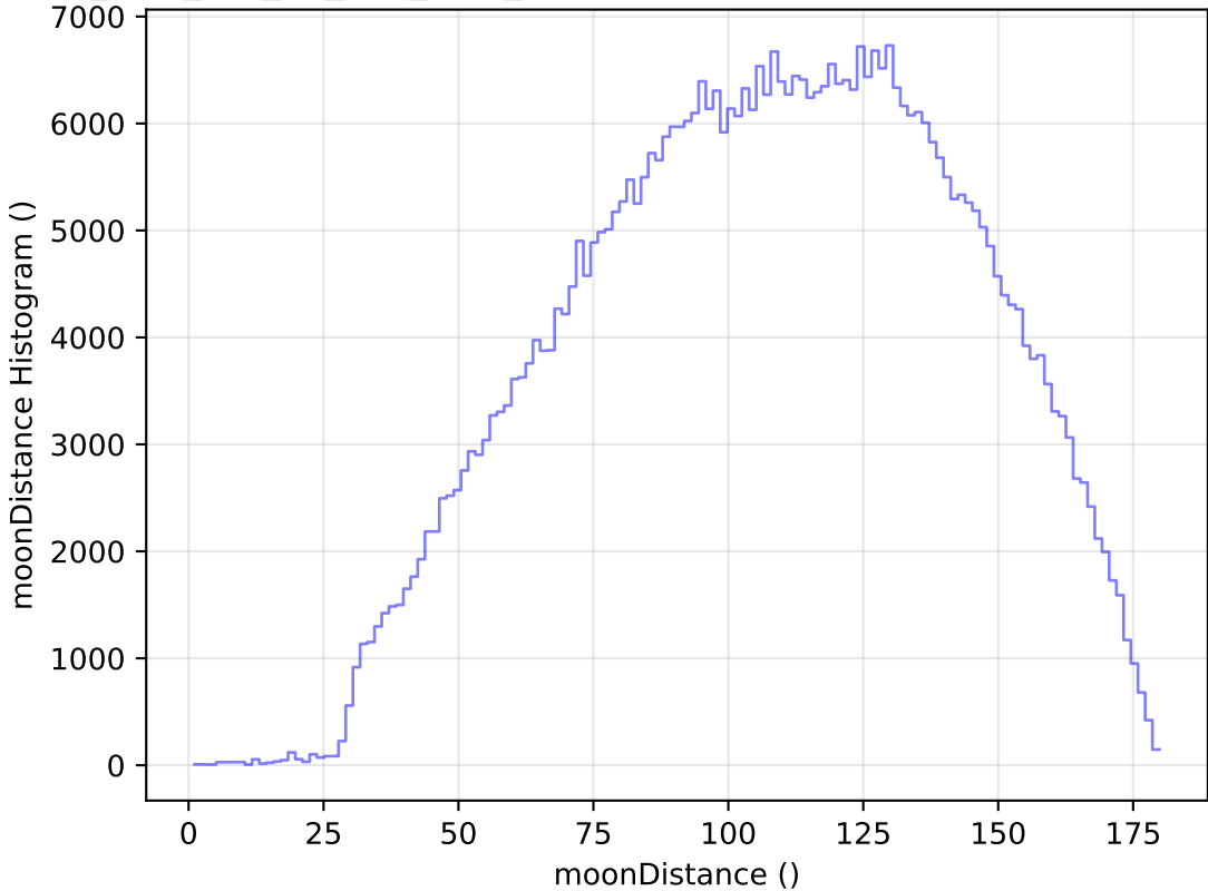
too_elab_r32_d2_griz_v3.4_10yrs WFD r band: moonDistance Histogram
