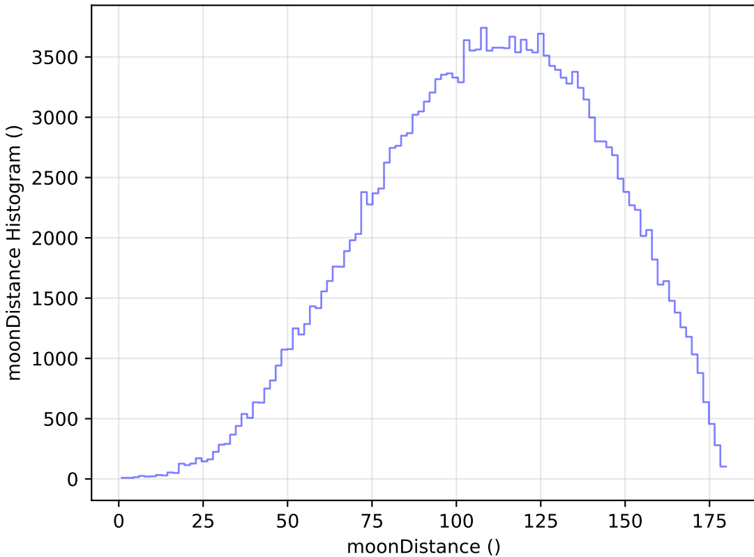
too_elab_r32_d2_griz_v3.4_10yrs WFD g band: moonDistance Histogram
