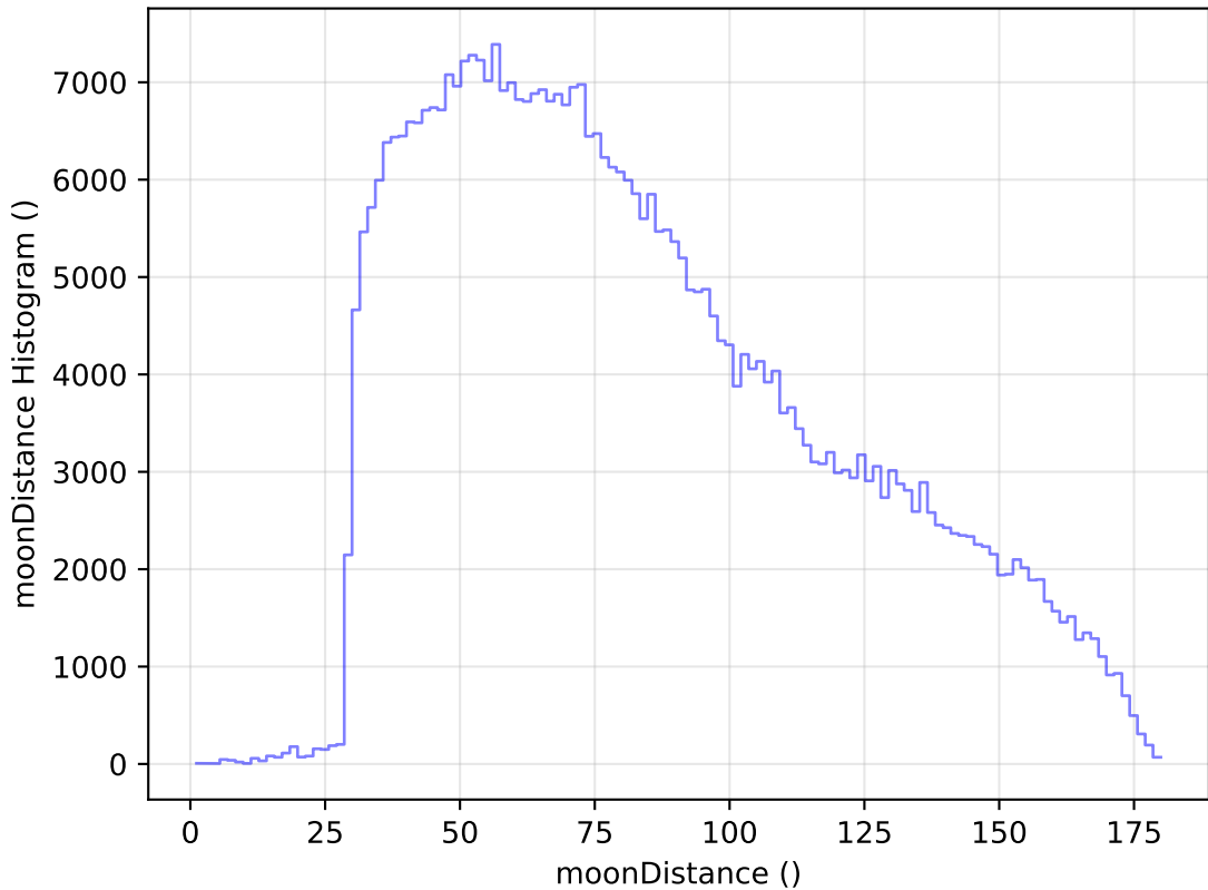
too_elab_r32_d2_griz_v3.4_10yrs All sky z band: moonDistance Histogram
