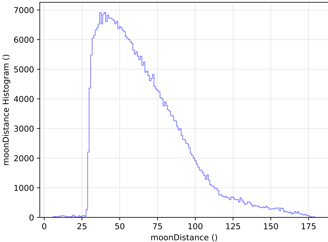
too_elab_r32_d2_griz_v3.4_10yrs All sky y band: moonDistance Histogram
