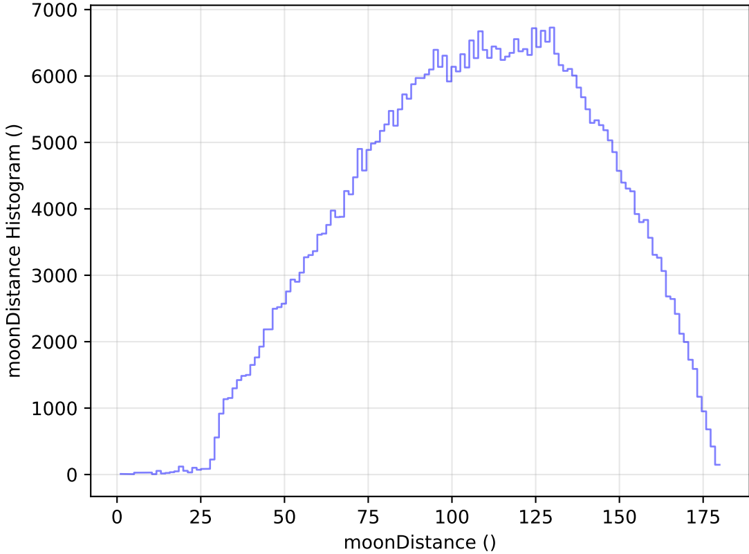
too_elab_r32_d2_griz_v3.4_10yrs All sky r band: moonDistance Histogram
