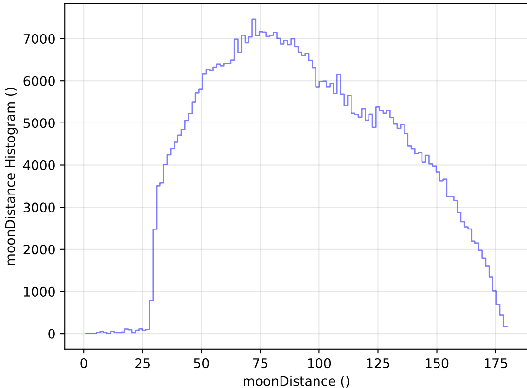
too_elab_r32_d2_griz_v3.4_10yrs All sky i band: moonDistance Histogram
