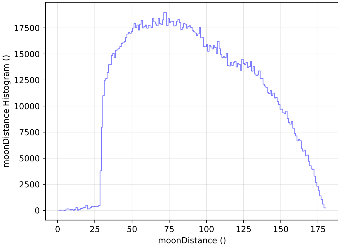
too_elab_r32_d2_griz_v3.4_10yrs All sky all bands: moonDistance Histogram
