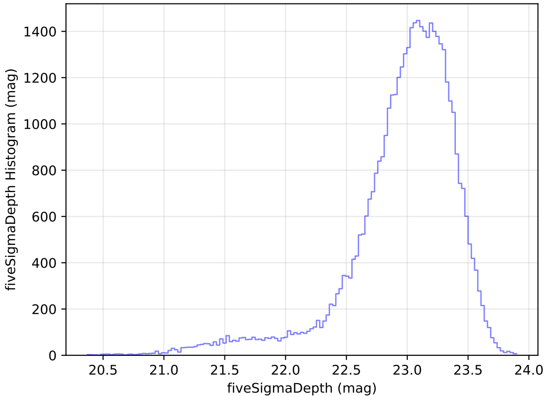
too_elab_r32_d2_griz_v3.4_10yrs Yr 1 z band: fiveSigmaDepth Histogram
