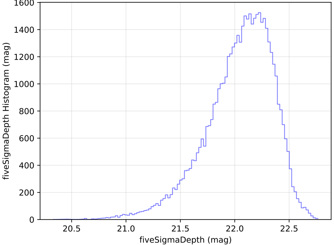
too_elab_r32_d2_griz_v3.4_10yrs Yr 1 y band: fiveSigmaDepth Histogram
