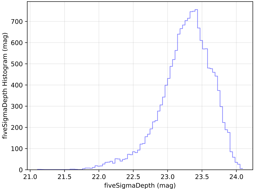
too_elab_r32_d2_griz_v3.4_10yrs Yr 1 u band: fiveSigmaDepth Histogram
